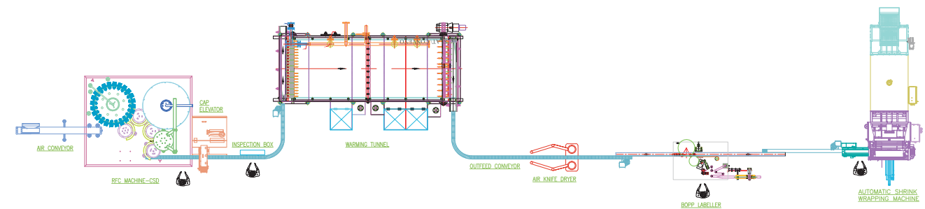
CARBONATED BEVERAGE PACKING LINE
